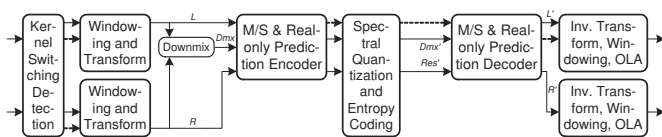
Figure 3.7. Joint-stereo transform coding using real-only prediction and kernel switching proposal in filter bank module.
