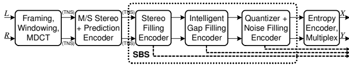
Figure 3.25. Detailed encoder of Fig. 3.23 with SBS in the JS domain. (---) parameter data. (TNS) is optional, and its application can vary in location.
