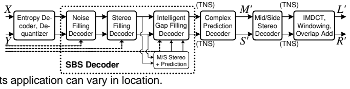
Figure 3.26. Detailed SBS enhanced USAC decoder of Fig. 3.23 associated with the encoder of Fig. 3.25.
